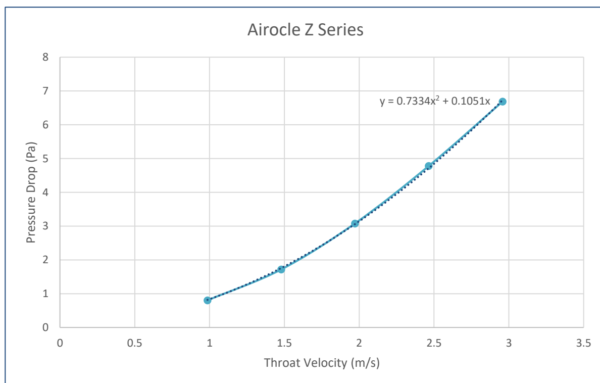
Figure 3: Z Series Pressure Drop Graph for a 1m X 1m Panel
