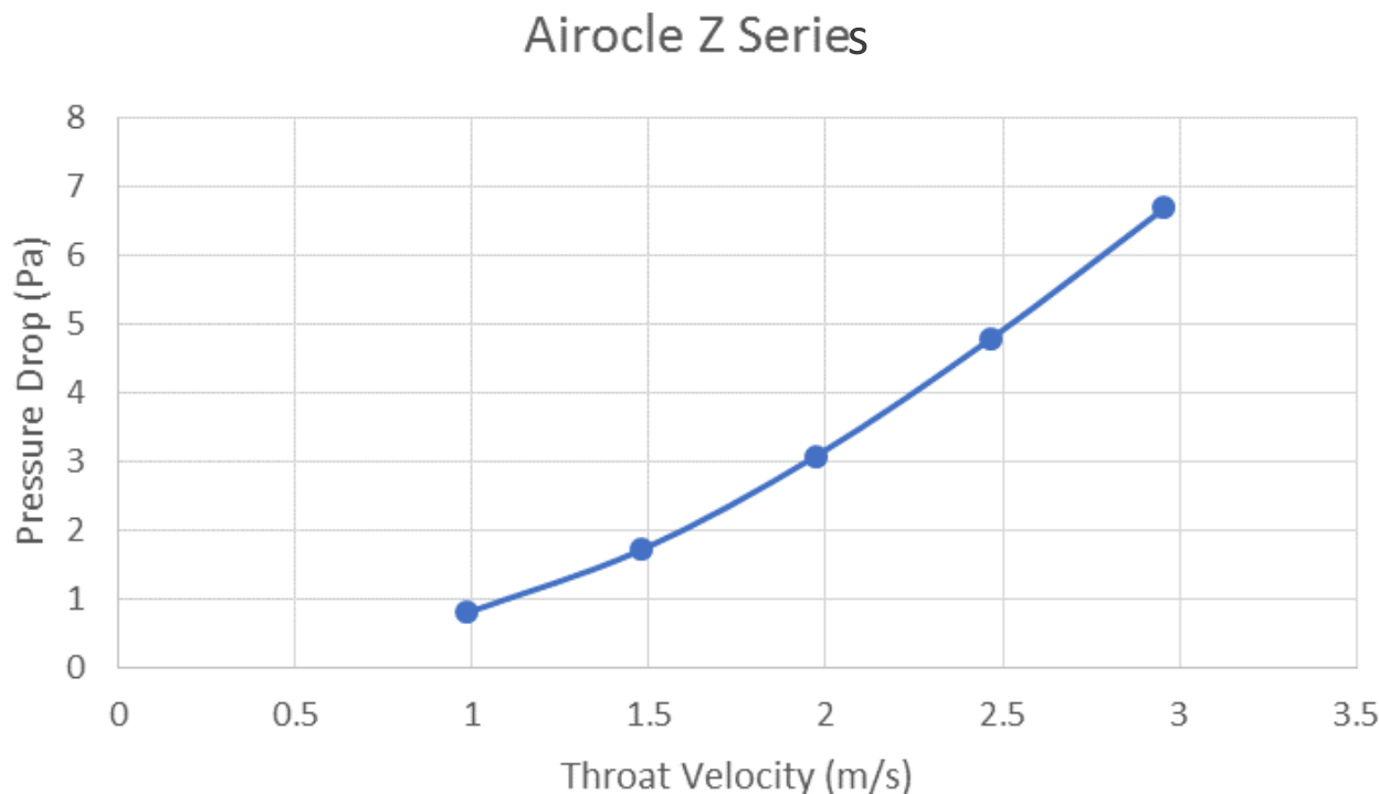
Figure 3: Z Series Louvre Pressure Drop Graph for a 1m H x 1m W Louvre Panel
